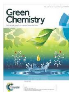
Green Chemistry
